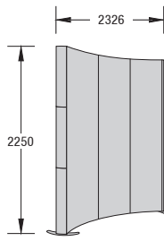
VA 5833 P1 for 3 panels aluminium side extrusions, silver anodized, incl. 2 spots
