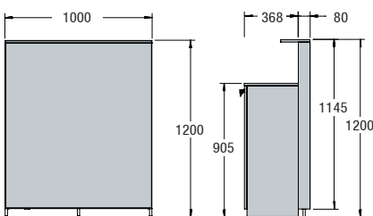
OCTALUMINA OL C400 OCTALUMINA Counter basic set incl. door set
