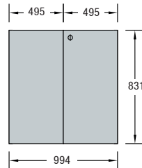
OL C480 Door set OCTALUMINA Counter
