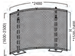
OP 200 Banner set curved concave 2 telescopic uprights and 4 beam extrusions 1240 mm long, incl. 2 base plates
