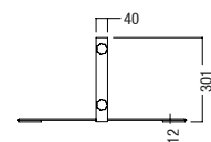
M 1951 Base plate, steel side, 600 x 250 mm
