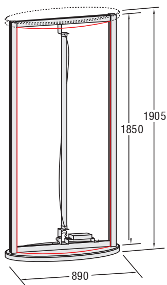
Panel size: W 800 x H 1850 mm
