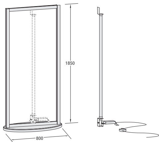
VA 7500 Basic set column base: wood, black supplied without panels
