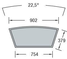
Q 400.30 Basic set, white
